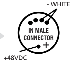
input connector rear side welding view
