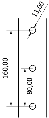
bracket MW 33
