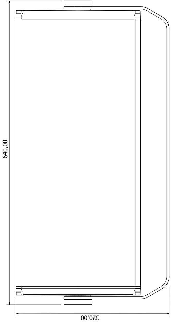
bracket MW 66
