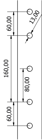
bracket MW 66
