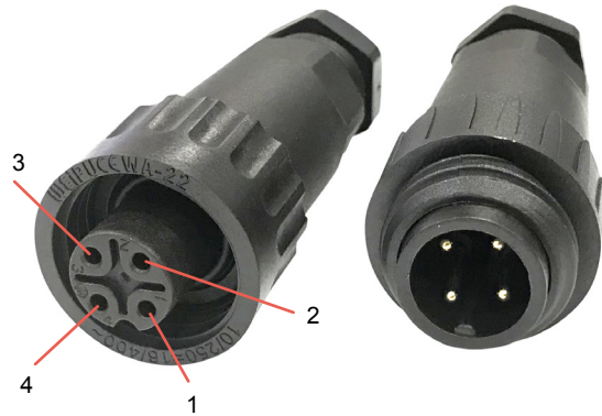
Female and Male 4 PIN connector / Connettore 4 PIN femmina e maschio
