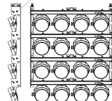
example of mounting with optional bracket for n.4 Parbar (art. JB4)
